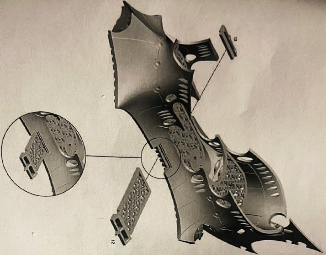
9. Right Wing Blade
